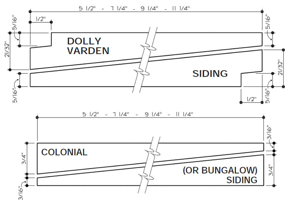
BEVEL SIDING PROFILES
