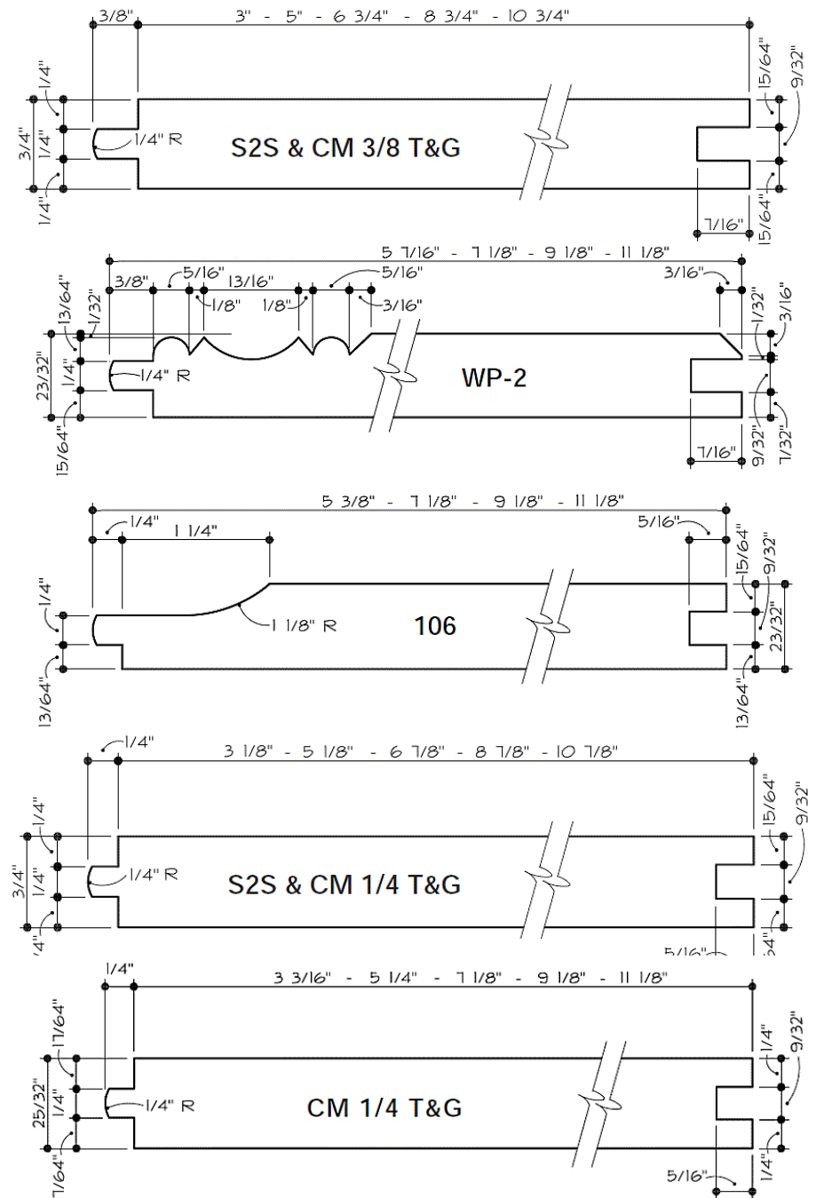
TONGUE & GROOVE SIDING AVAILABLE PROFILES
