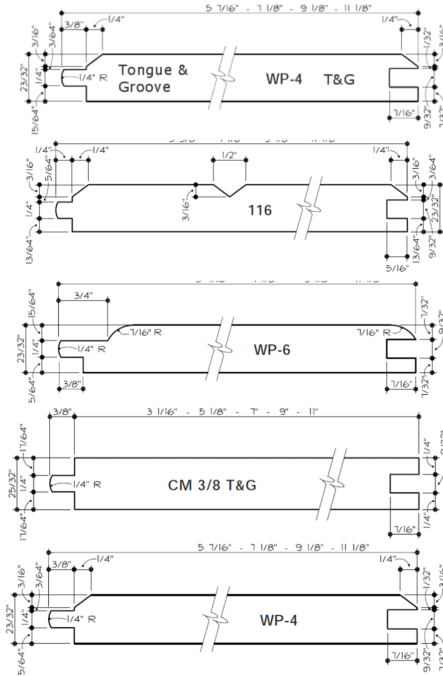
TONGUE & GROOVE SIDING AVAILABLE PROFILES
