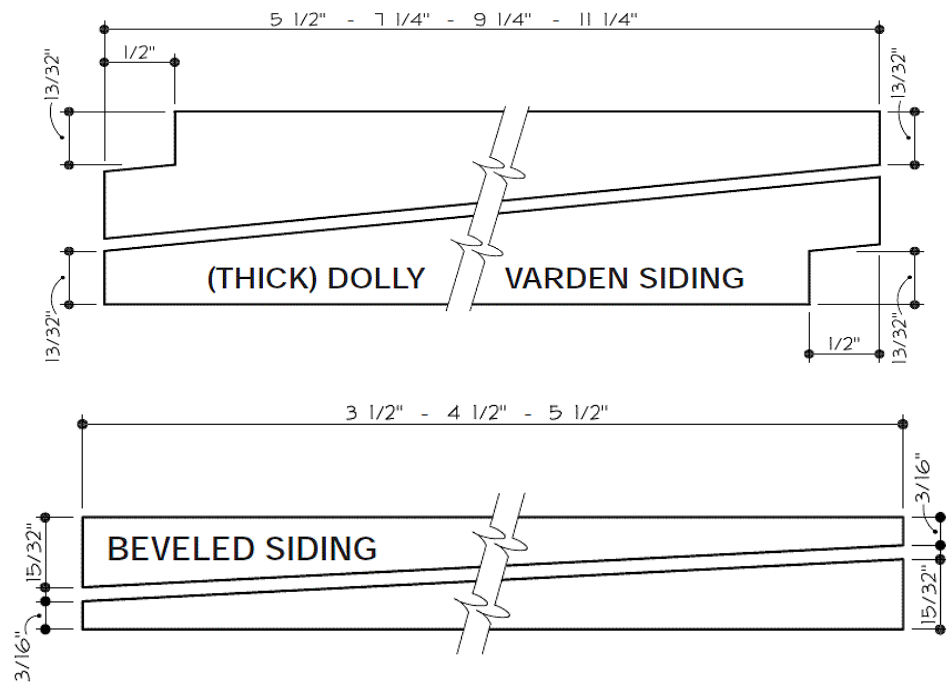
BEVEL SIDING PROFILES
